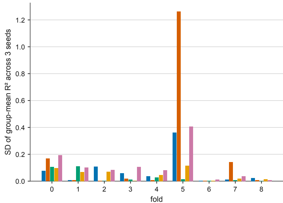
IP — per-fold instability
